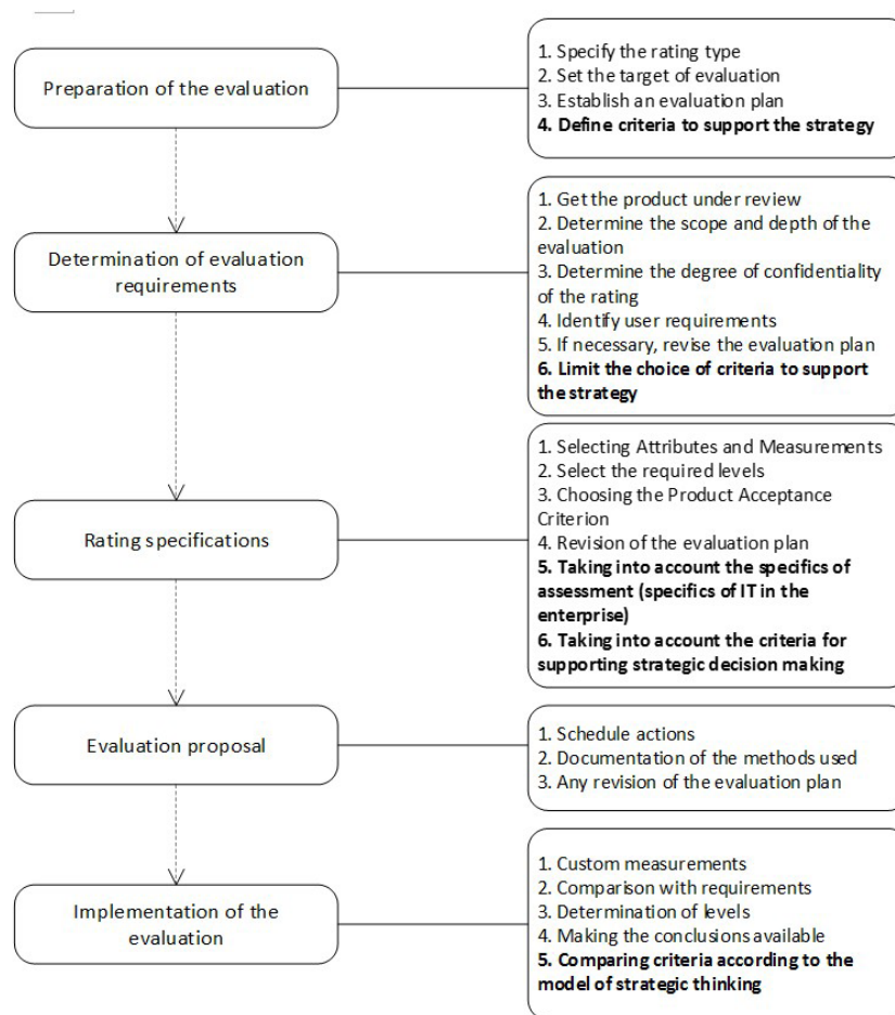
Figure 3: Diagram of a modified reference model for evaluating the quality of SW with support of strategic decision-making.
